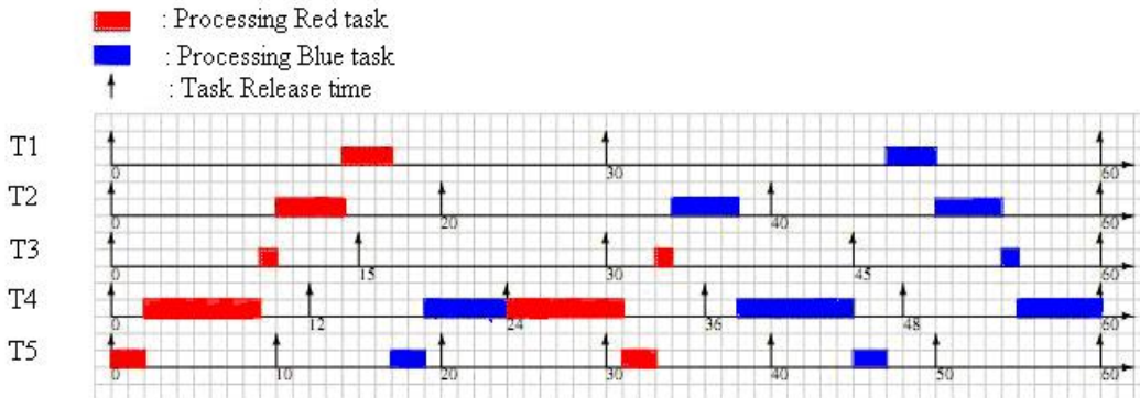
Figure 2: BWP schedule ( sf_j = 2 )
