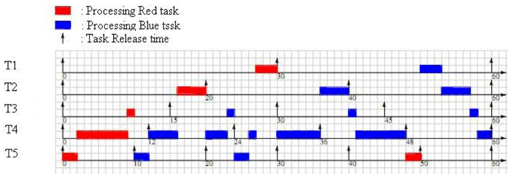
Figure 3: RLP Schedule ( sf_i = 2 )
