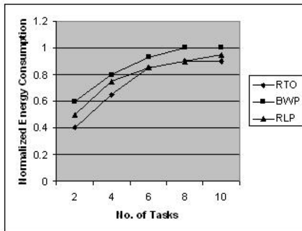
Figure 6. Normalized Energy Consumption
