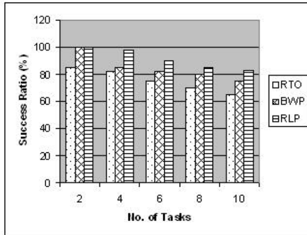
Figure 5. Success Ratio
