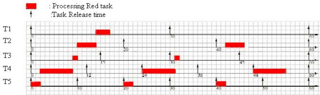
Figure 1: RTO Schedule ( sf_i = 2 )
