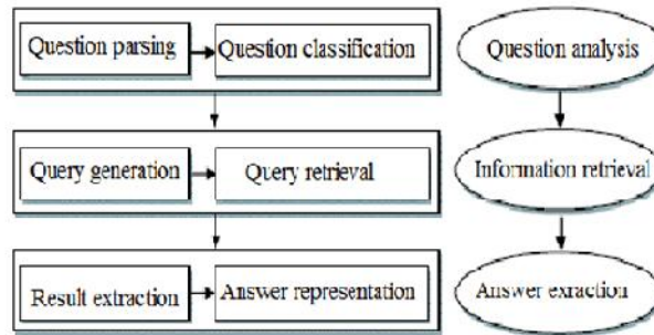
Figure 1. Generic Text-based Question Answering System
